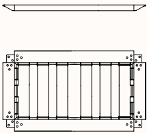
Frame with Elastic Belt for Seat U85 OW 800mm OD 450mm OH 40mm
