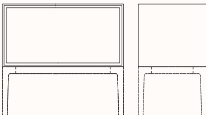
Cabinet U81 / U91 OW 800/900mm OD 450mm OH 740mm
