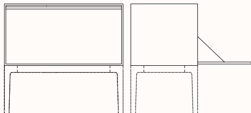
Cabinet with Drop Down Door U81_R/U91_R OW 800/900mm OD 450mm OH 740mm
